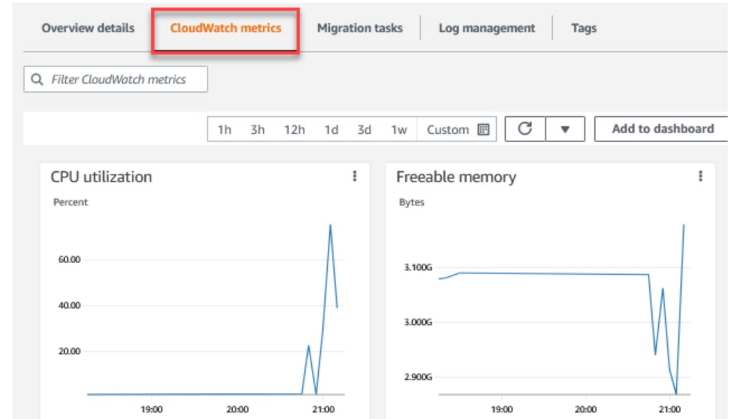
Host Metrics
